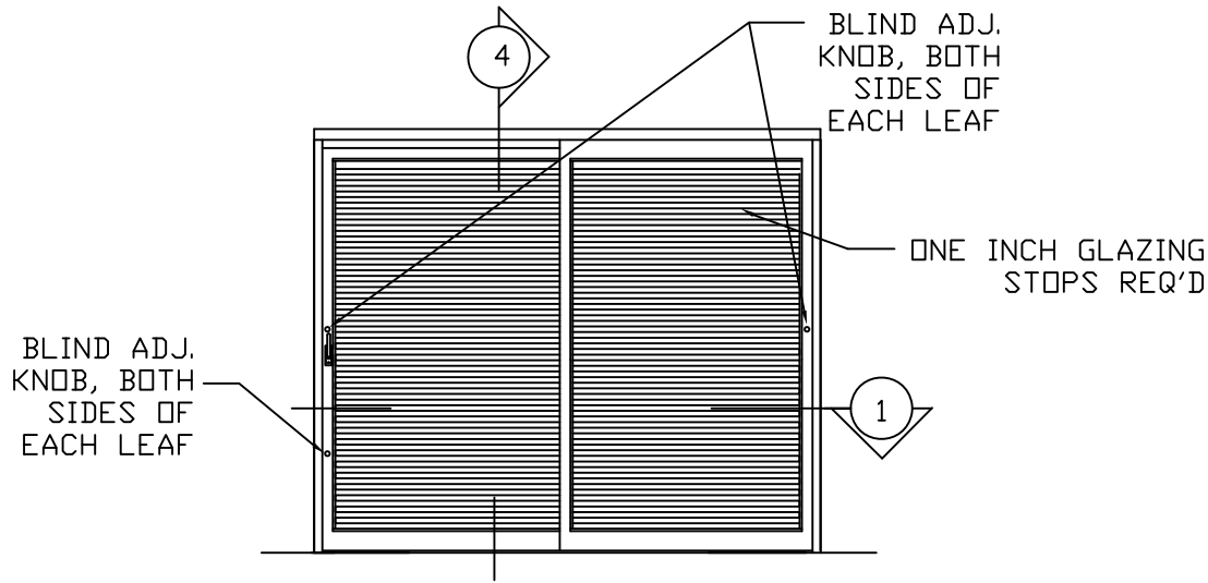
ROOM SIDE ELEVATION
